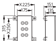
Distance between centers 40, 50 and 60 mm
