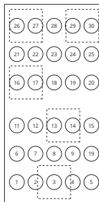
Distance between centers 50 mm
