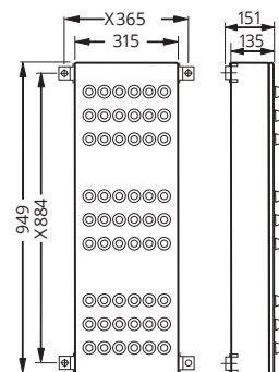
Distance between centers 60 mm
