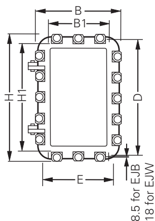
Ex-Enclosure IIB metal enclosure
