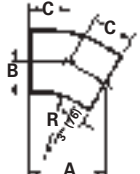
30° Horizontal Bend
