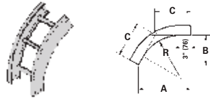
60° Vertical Outside
