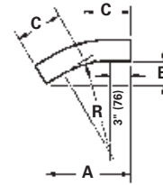
30° Vertical Outside
