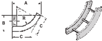
60° Vertical Inside
