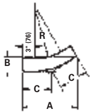
30° Vertical Inside
