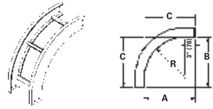
90° Vertical Outside
