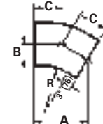
30° Horizontal Bend
