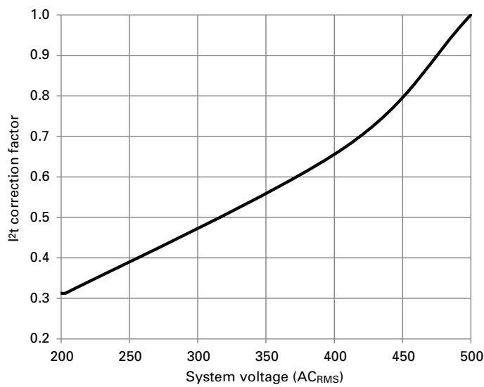
AC clearing I²t voltage correction factor
