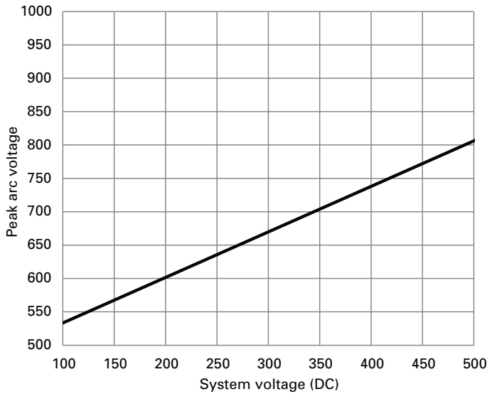
DC arc voltage
