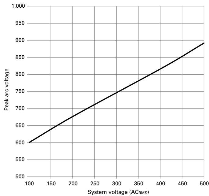
AC arc voltage
