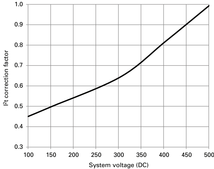
DC clearing I²t voltage correction factor
